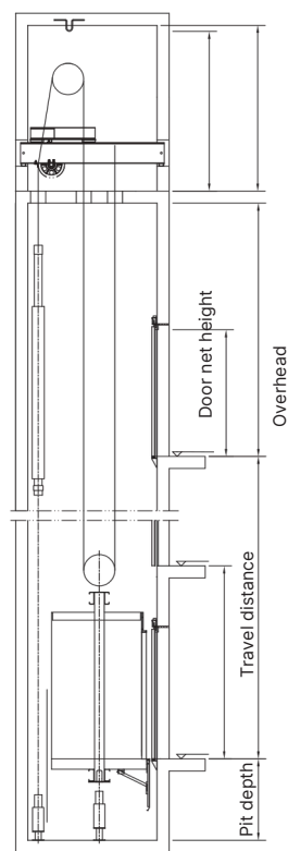
Counterweight rear side view of the shaft
