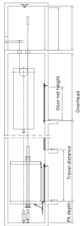
Counterweight side side view of the shaft
